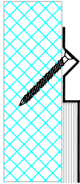
(B) (1" - 2" EJ)
