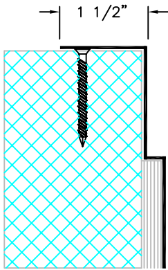
(E) (1" - 2" EJ)
