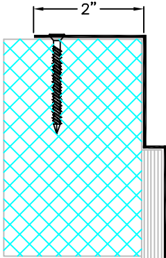
(A) (1" - 2" EJ)
