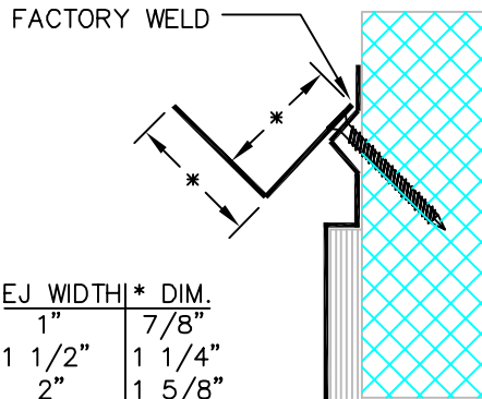
(F) (1" - 2" EJ)
