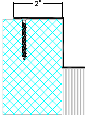
(C) (3" - 18" EJ)
