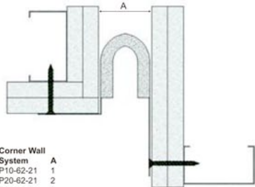
Corner Wall / Ceiling to Wall
