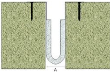
Floor to Floor / Roof to Roof
